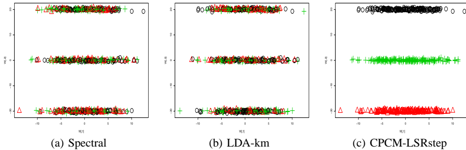
Figure 2: Comparison of Spectral, LDA-km and CPCM on a simulated dataset.
