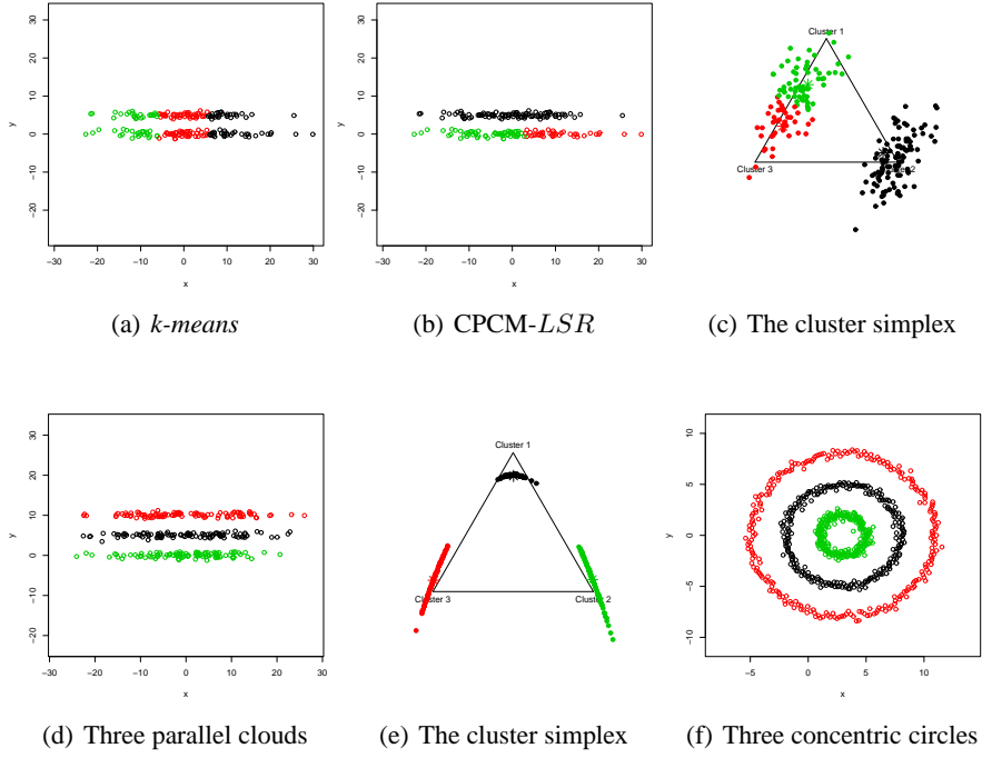
Figure 1: An example run is shown from (a)-(c). Data is from two parallel lines with Gaussian noise. (a) K -means creates parallel vertical bands to reduce the within cluster variance, and fails to cluster “correctly.” Blur ratio for K = 3 , BR_3 = 0.26 and for K = 2 , BR_2 = 0.447 (b) In contrast, CPCM finds the underlying elongated band structure. Blur ratio for K = 3 , BR_3 = 0.148 and for K = 2 , BR_2 = 0.041 . Thus, blur ratio is indeed minimized by CPCM for the right number of clusters. (c) Linear regression transforms the data linearly on to the simplex. Examples using CPCM-RKHS with a Gaussian kernel are shown from (d)-(f). (d) Three parallel lines (e) Projection on the simplex space shows that CPCM tries to pull the cluster centers to the simplex corners. (f) Three concentric circles.
