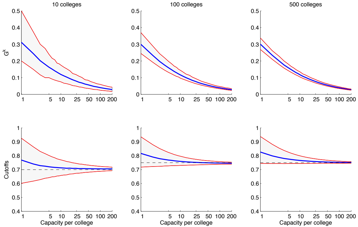
FIGURE 4. Speed of convergence
