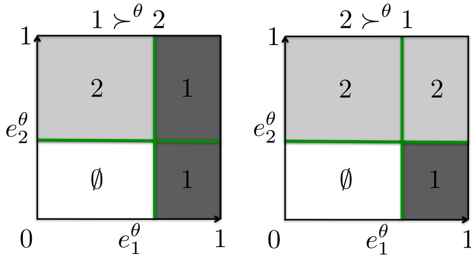
FIGURE 2. A stable matching in a continuum economy with two colleges
