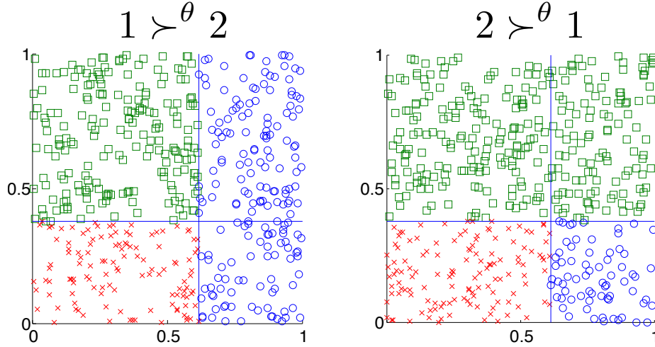
FIGURE 3. A stable matching in a discrete economy approximating the example.
