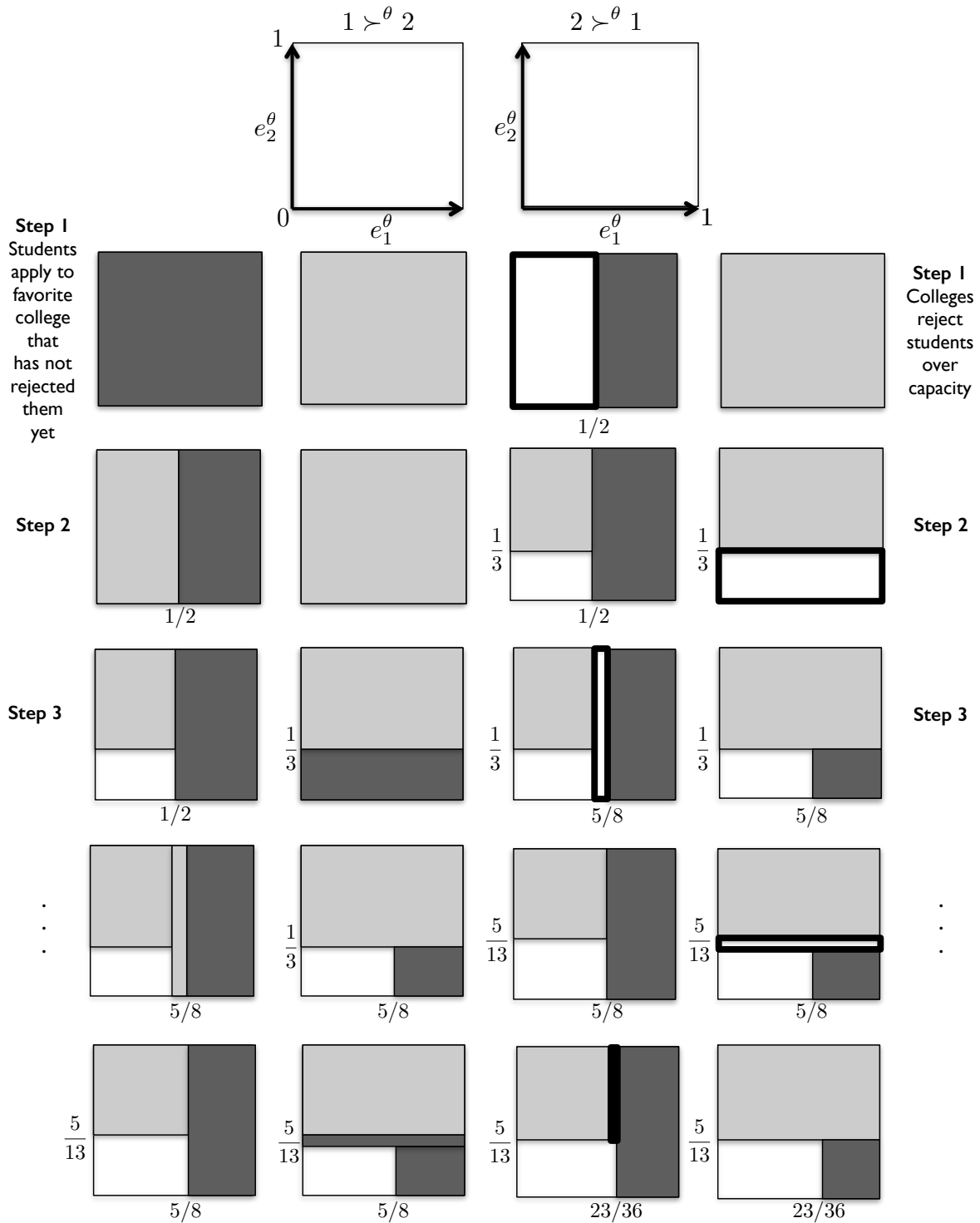
FIGURE 1. The Gale and Shapley algorithm
